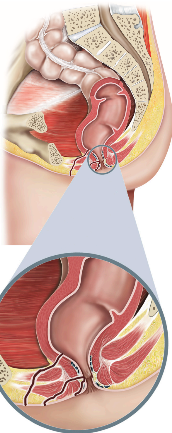
Figure 1 Different positions of an anal fistula
